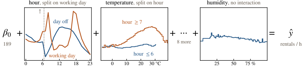
Figure 1: A CALM fitted on the Bike Sharing dataset: the prediction sums one plot per feature, each plot holding one curve per region. The hour splits on the working day; the temperature splits on the hour, mattering by day and barely at night; the humidity interacts with no feature and keeps one curve. The dotted line on the hour’s plot marks where the temperature’s and the year’s regions switch and its arrow gives the sign of the hidden jump; Section 3.2 explains it in depth.
