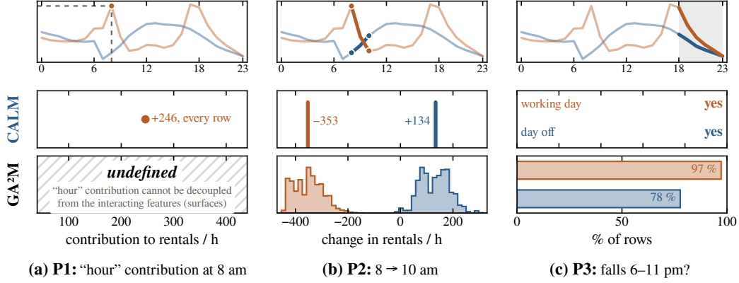
Figure 3: The three properties on the model of Figure 2, each asked on every row of the data. Top: CALM’s curves, the question marked. CALM’s answers are read by eye; the GA 2 M’s are computed, each of the 17,379 rows through its eight terms with the hour. (a) The hour’s contribution at 8 am on a working day: CALM reads +246 off the working-day curve, the same on every row; the GA 2 M’s is undefined, since the hour’s contribution cannot be decoupled from the interacting features (its seven surfaces). (b) \hat{y}(10 \text{ am}) - \hat{y}(8 \text{ am}) : CALM -353 on working days and +134 on days off, exact on every row since no dotted line is crossed; the GA 2 M spreads from -430 to -257 and from +54 to +215 (5th–95th percentile). (c) Does the prediction fall every hour from 6 pm to 11 pm? CALM: yes on working days and days off, since both curves fall and cross no dotted line; the GA 2 M: on 97% of working days and 78% of days off.
