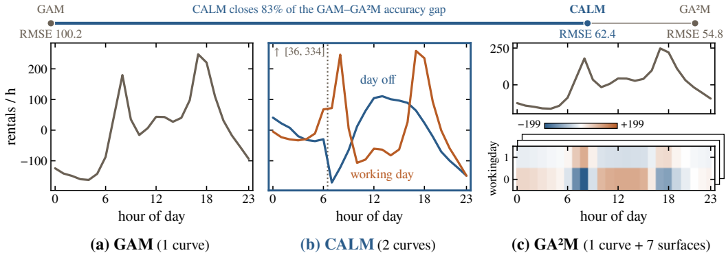
Figure 2: The effect of the hour on bike rentals (Bike Sharing dataset). Top: test RMSE (Table 5); CALM closes 83% of the gap from GAM to \text{GA}^2\text{M} . (a) GAM: one curve. The interaction with the working day is averaged away, which limits accuracy. (b) CALM: one curve for working days and one for days off (at d_{\max} = 1 ). The dotted line mark a hidden jump (see Section 3.2 for more details). (c) \text{GA}^2\text{M} : a curve and seven 2D surfaces (only one shown here) for decoding the effect of the hour, which limits its interpretability.
