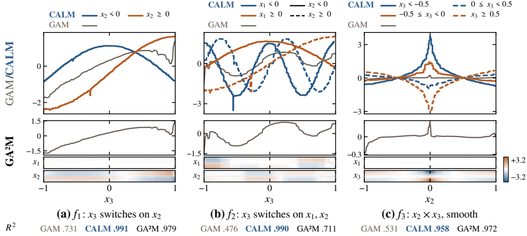
Figure 4: Cases 1 to 3 (one column each) of Section 4.1. Top: CALM’s curves, one per region, over the GAM’s single curve (gray). Bottom: the GA²M’s main curve alongside its two heatmaps. Under each column: the mean R^2 over 5 folds (Table 3), with CALM at depth 2; f_1 ’s panel is drawn at depth 1.
