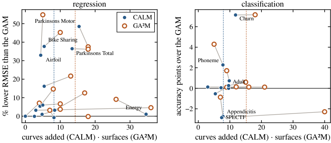
Figure 6: What each model asks a reader to inspect beyond the GAM’s one curve per feature, against what it gains over the GAM (24 datasets, Electrical excluded; means over 5 folds). For CALM the count is its splits, each of which adds one curve; for the GA 2 M it is its pairwise surfaces. One dot (CALM) and one ring (GA 2 M) per dataset, joined; dotted lines mark the means. CALM inspects 8.2 added curves on average against 14.3 surfaces in regression and 7.9 against 15.2 in classification, and recovers about 60 % of the GA 2 M’s gain where that gain exceeds one point. Significance is marked in Tables 4 and 5.
