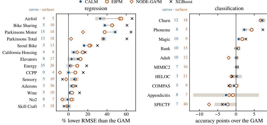
Figure 5: What each model gains over the GAM on each dataset: the black box XGBoost, the GA 2 Ms NODE-GA 2 M and EB 2 M, and CALM (means over 5 folds, higher is better). The gray band behind each dot is \pm \max(\text{std}_{\text{CALM}}, \text{std}_{\text{EB}^2\text{M}}) over the folds. A ring inside it is a draw, outside a win or a loss. CALM ahead/level/behind: against the GAM, 8/6/0 in regression and 3/7/0 in classification; against EB 2 M, 1/5/8 and 0/7/3 (see Tables 4 and 5 for full results). Left of each row: the curves that CALM adds on top of the GAM, and the pairwise surfaces that EB 2 M fits.
