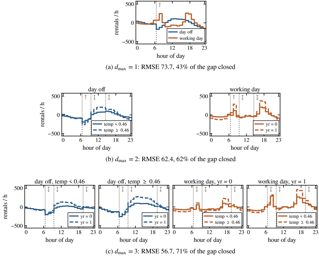
Figure 7: What depth buys: the hour of the Bike Sharing data under CALM at d_{\max} = 1, 2 and 3 (fits on all rows; depth 1 is the model of Figure 2, depth 2 the default of Table 5). Each level splits every region once more, giving 2, 4 and 8 curves: (a) shows both, (b) one panel per day type and (c) one panel per region of the first two splits, each panel above the two it splits into; the hue is the day type, the line style the last split; dotted lines mark where another feature’s region switches on the hour, each with the sign of its hidden jump (§3.2): \uparrow [36, 334] at depth 1; \uparrow [8, 267] , \downarrow [-159, 63] and \downarrow [-48, 70] at depth 2; all three \downarrow at depth 3. Under each depth, the held-out RMSE of that depth and the share of the GAM \rightarrow XGBoost gap it closes, over 5 folds (GAM 100.2, XGBoost 39.4): 43 %, 62 % and 71 %.
