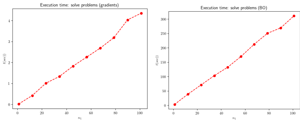
Figure 18: Execution time for defining and solving the optimisation problems. We observe that the Bayesian optimisation scheme is much more expensive, performing the task slower by a factor of 75.
