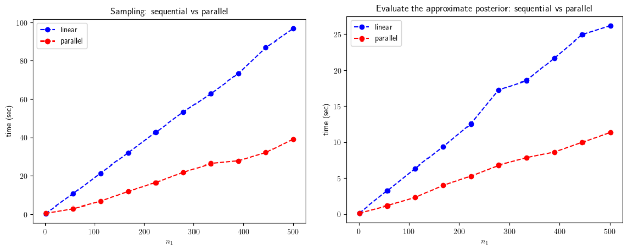
Figure 23: Execution time of the inference part exploiting parallelisation. At the left figure, we measure the execution time for sampling n_2 = 50 points per region. At the right figure we measure the execution time for evaluating the posterior at a batch of 50 points.
