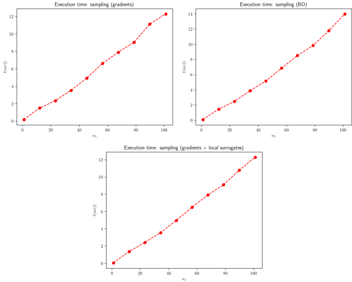
Figure 21: Execution time for sampling from the approximate posterior. We observe a small speed-up using the local surrogate model.
