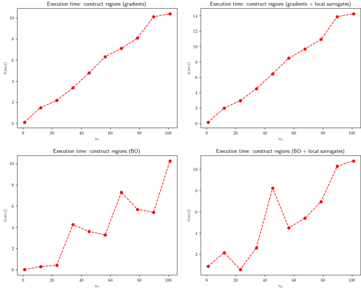
Figure 19: Execution time for constructing the n -dimensional bounding box region and, optionally, fitting the local surrogate models. We observe that fitting the surrogate models incurs a small increase by a factor of 1.5.
